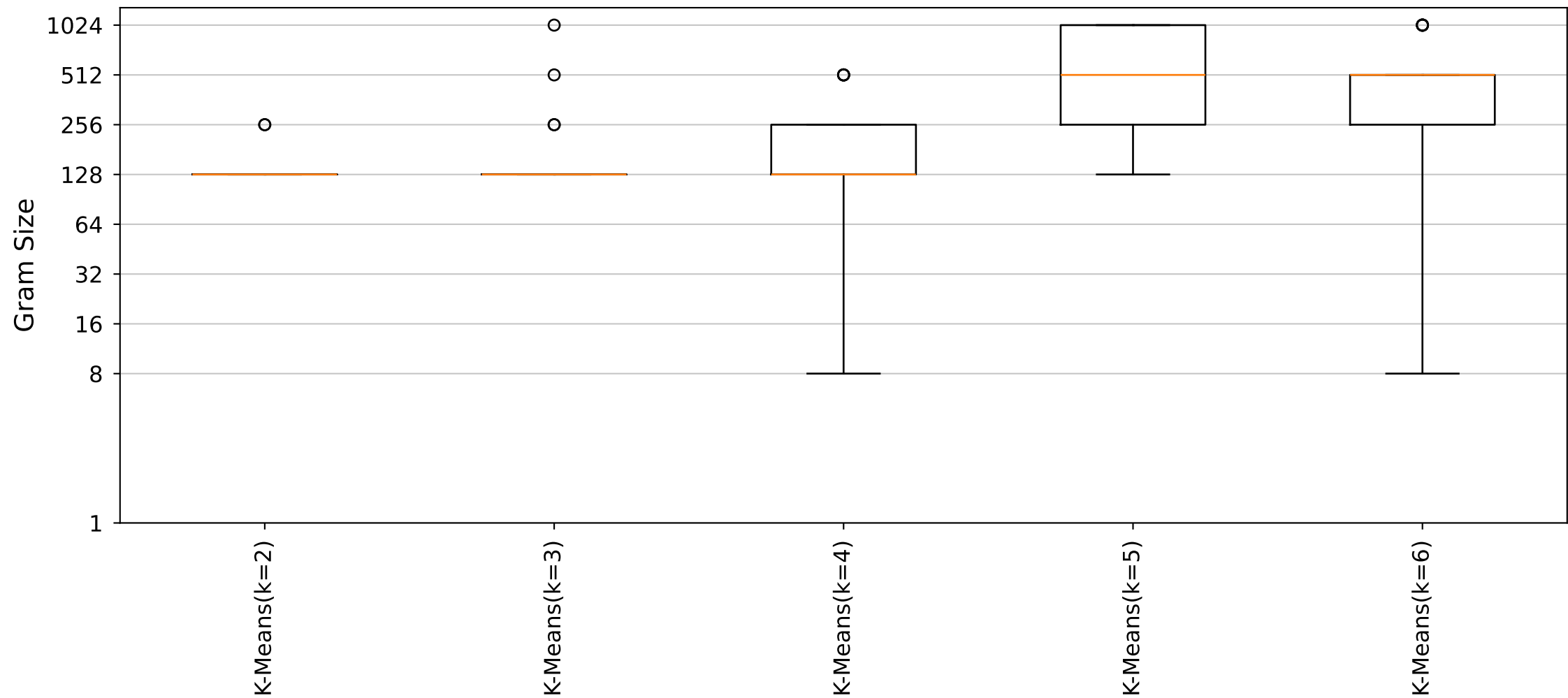
YARA Rules Gram Size Distribution (Cluster22_Size6 dataset)
